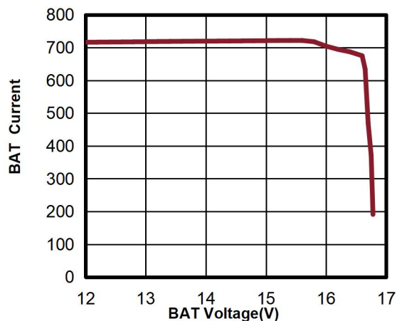
Figure 8.1.b R_{ICHG}=1.3K , 恒流和恒压充电电流
