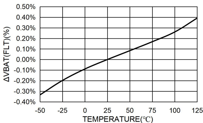
Figure 8.3.a Battery Float Voltage vs Temperature
