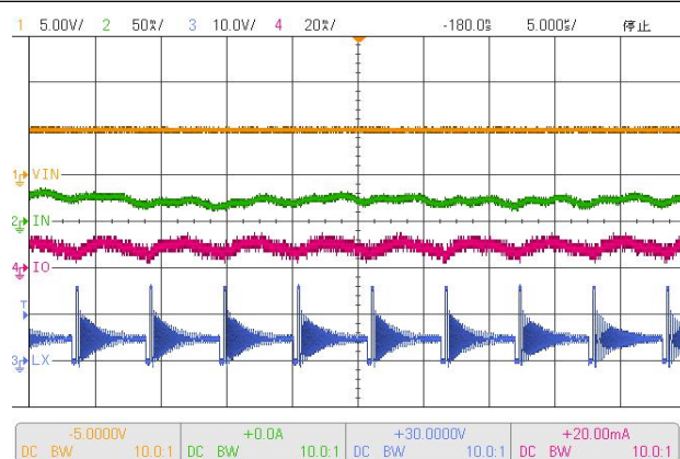
Figure 9.2 自适应限流
