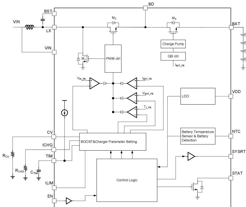
Figure 5. Internal function block diagram
