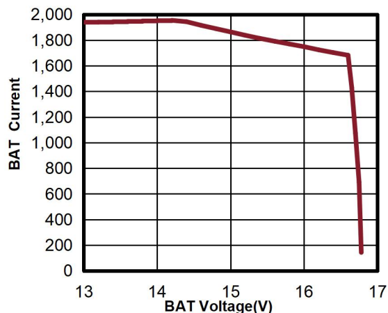
Figure 8.2.b R_{ICHG}=0.5K , 恒流和恒压充电电流
