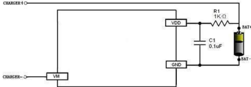
Fig 6 XR2150A in a Typical Battery Protection Circuit
